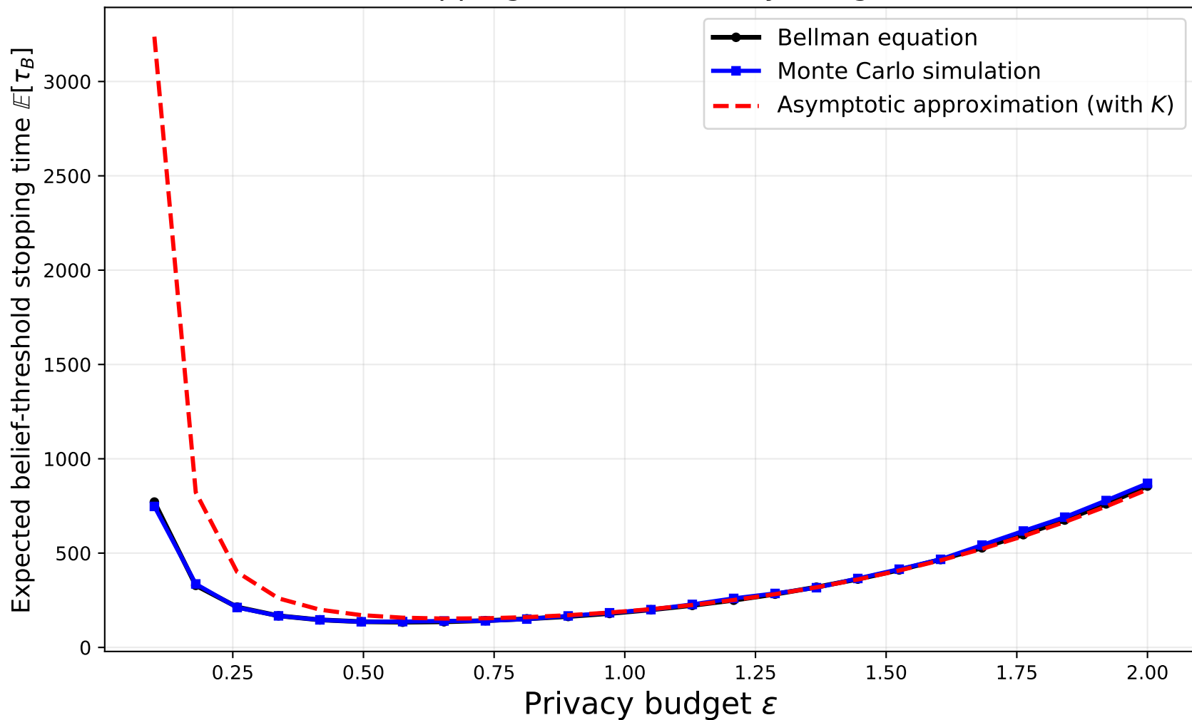
Belief-Threshold Stopping Time vs. Privacy Budget, B = 10.0 , \sigma = 1.0
