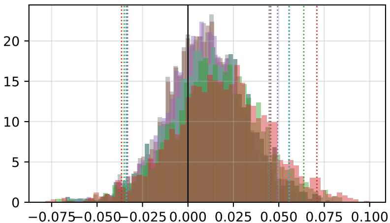
W-ind — 10-trading-day blocks
