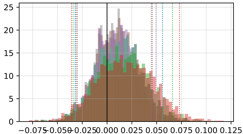
W-ind — 40-trading-day blocks
