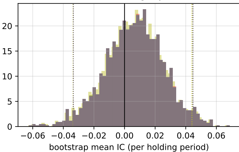
W-ind — 10-trading-day blocks
