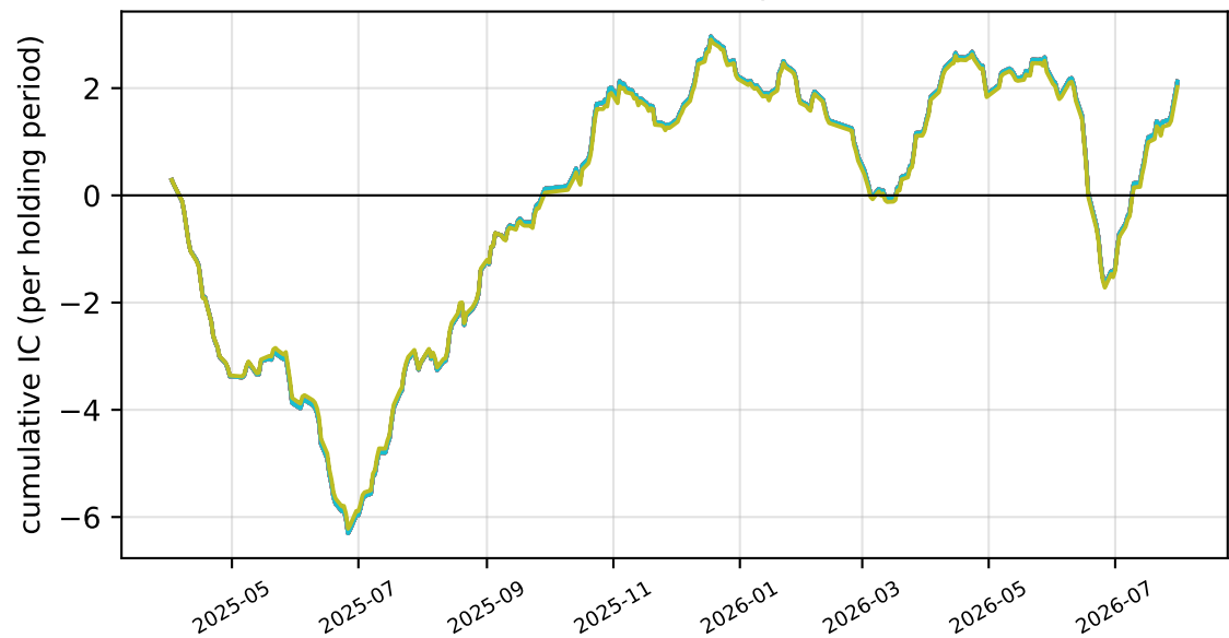
w-ind — cumulative daily IC (h=20d)
