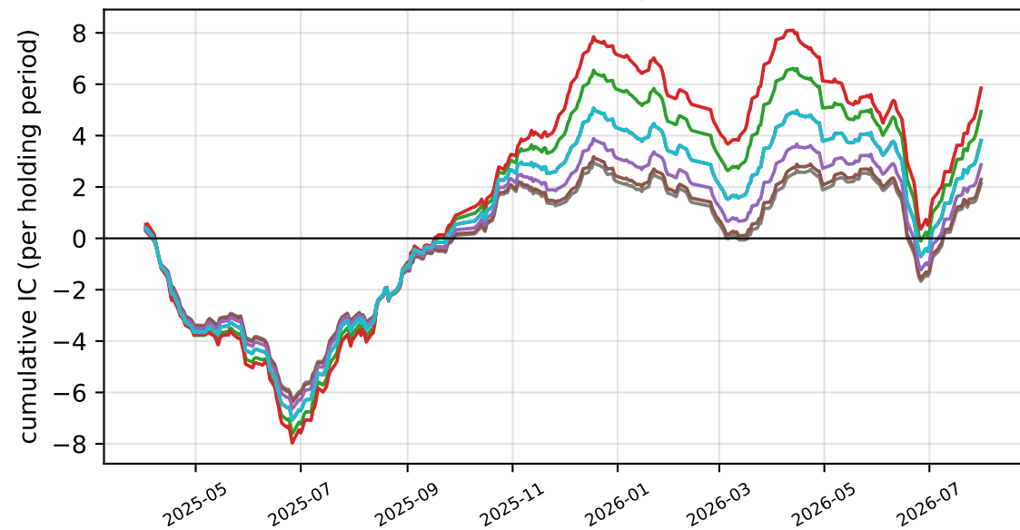
W-corr — cumulative daily IC (h=20d)
