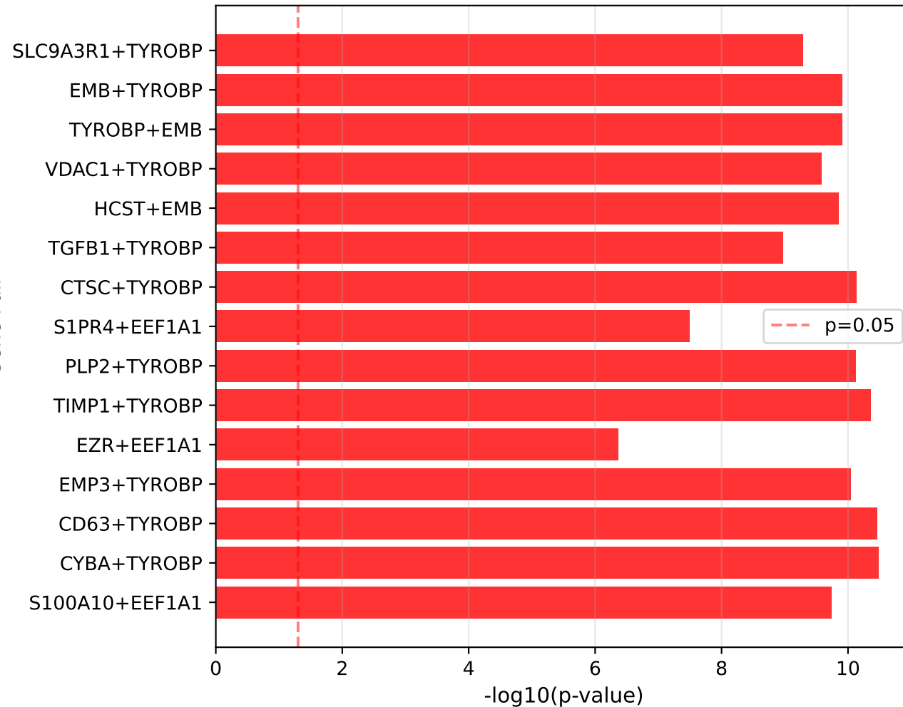
Statistical Significance (Wilcoxon Test)
