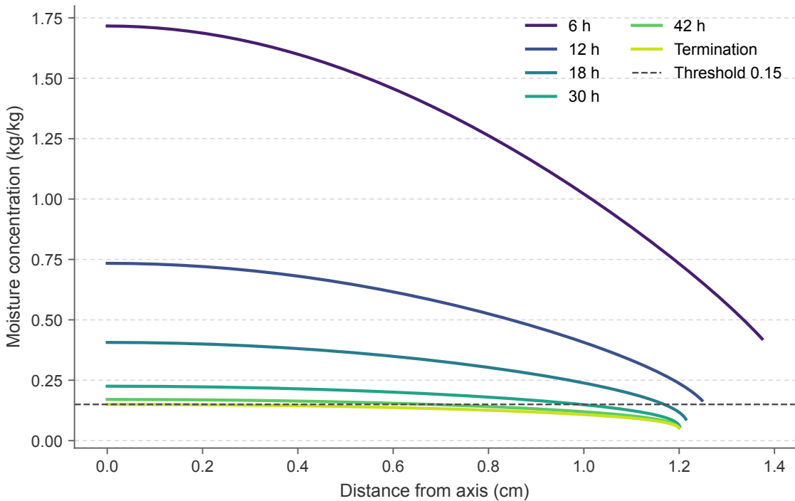
Radial moisture profiles with moving boundary
