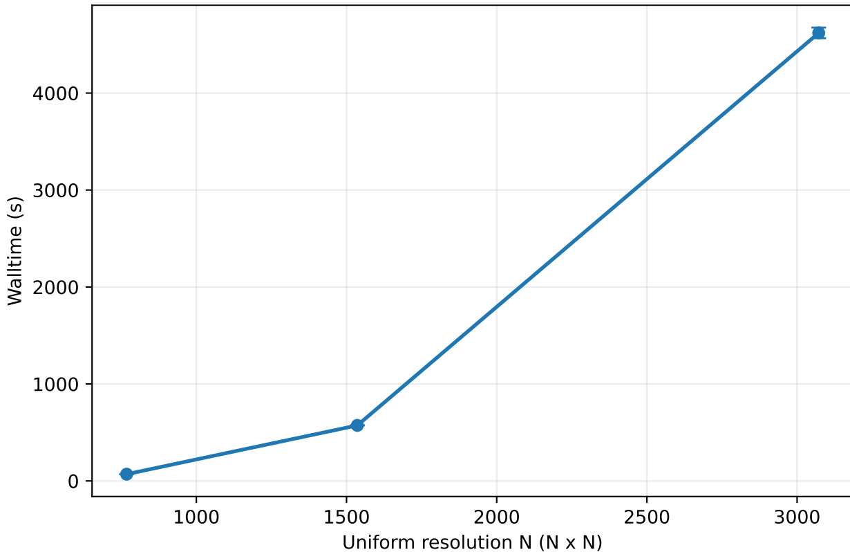
Task 3: Uniform No-AMR Serial Runtime vs Resolution
