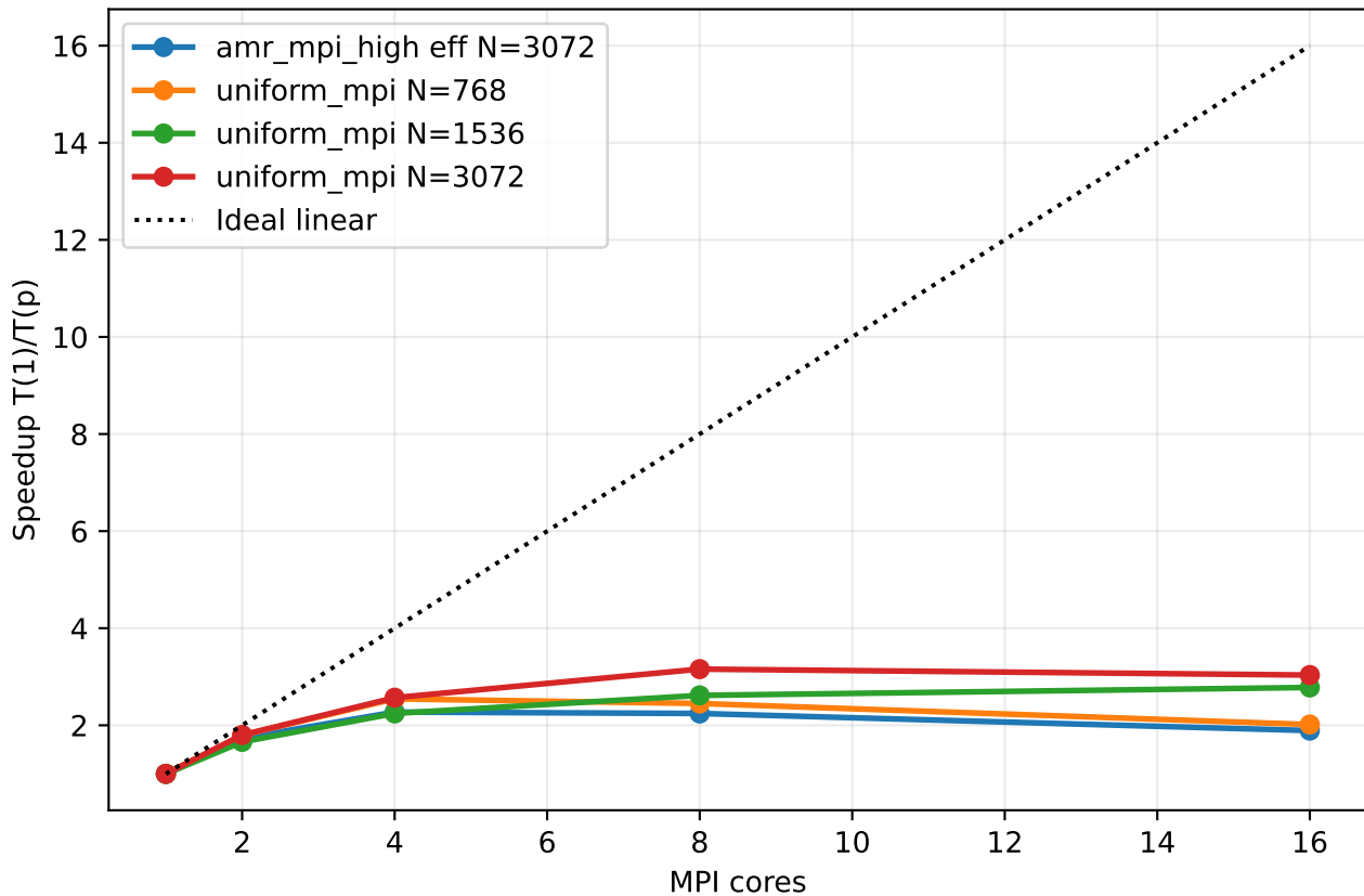
Task 3: Speedup vs Cores
