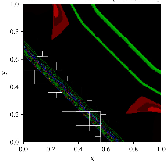
Toro test 4, diagonal split, AMR (base 200x200, max_level=1) \rho , t = 0.035 , fixed scale [0.455, 6.283]
