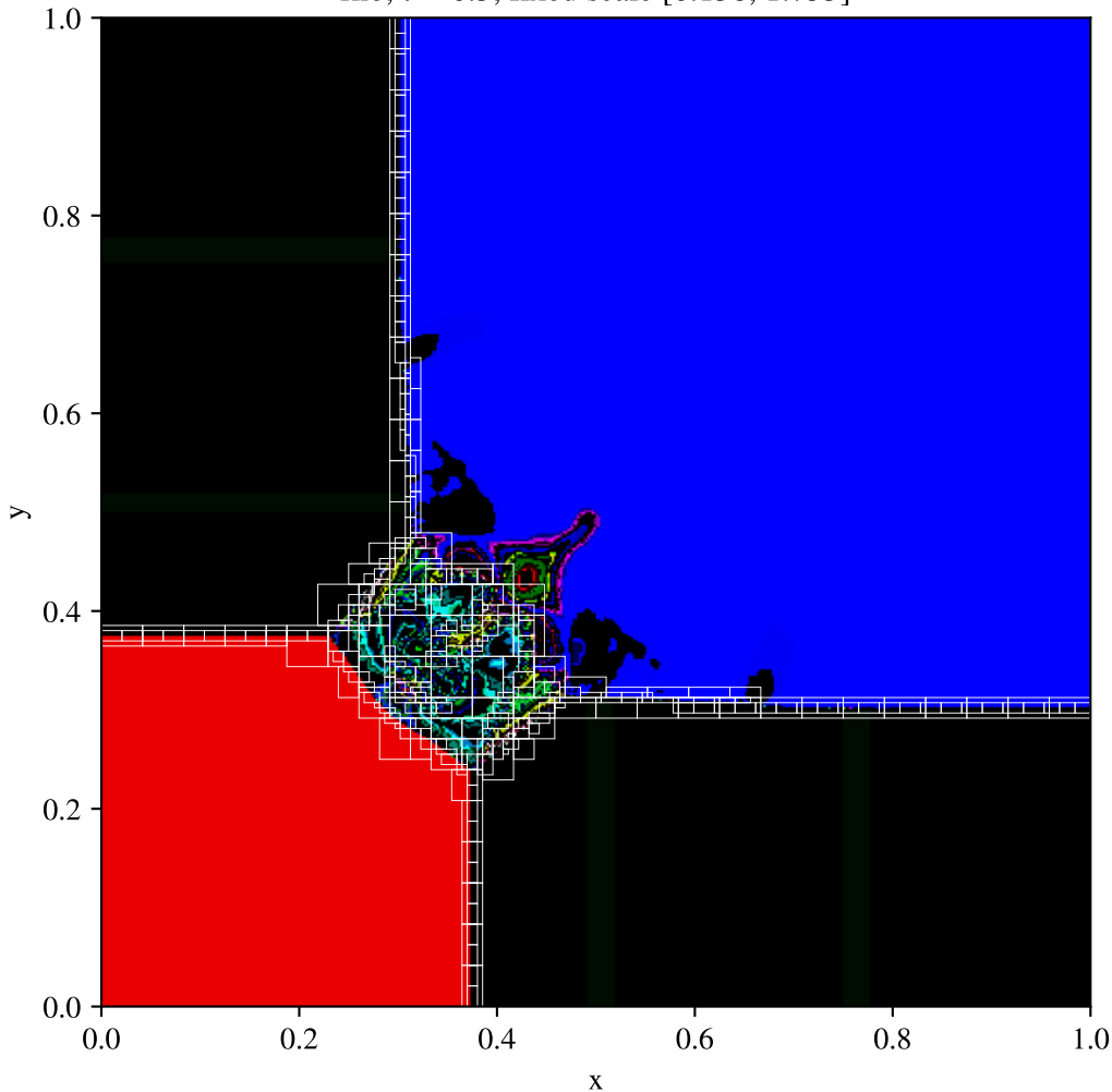
Task 3 quadrant benchmark, AMR serial effective N=3072 \rho, t = 0.3 , fixed scale [0.138, 1.753]
