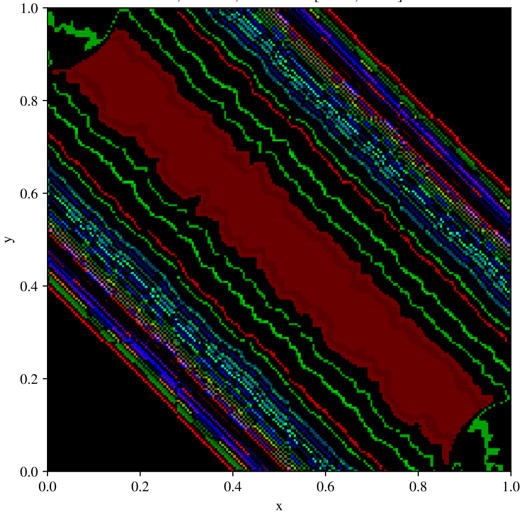
Toro test 2, diagonal split, AMR (base 200x200, max_level=1) \rho , t = 0.15 , fixed scale [0.015, 1.000]
