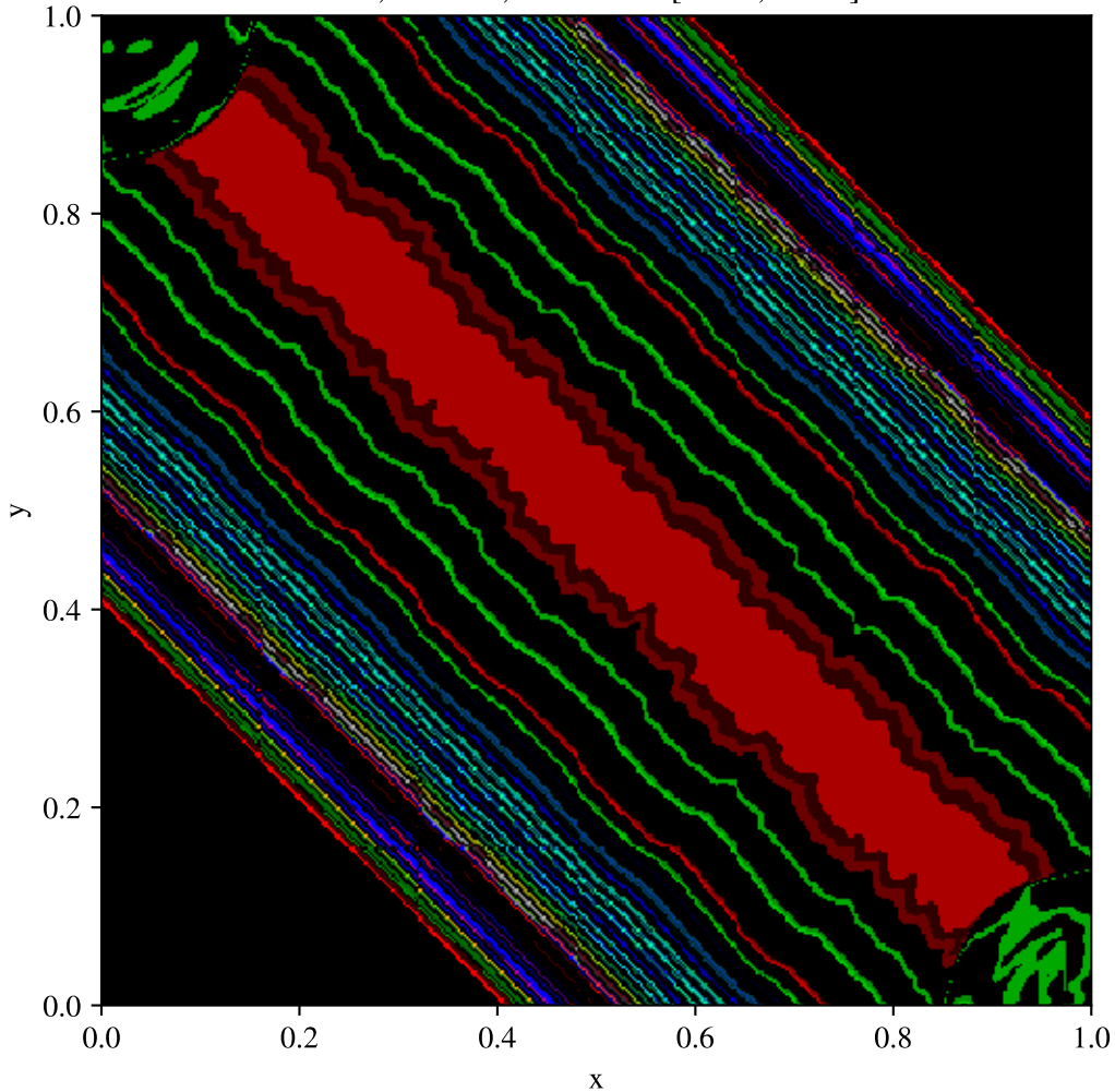
Toro test 2, diagonal split, Uniform (400x400) \rho , t = 0.15 , fixed scale [0.015, 1.000]
