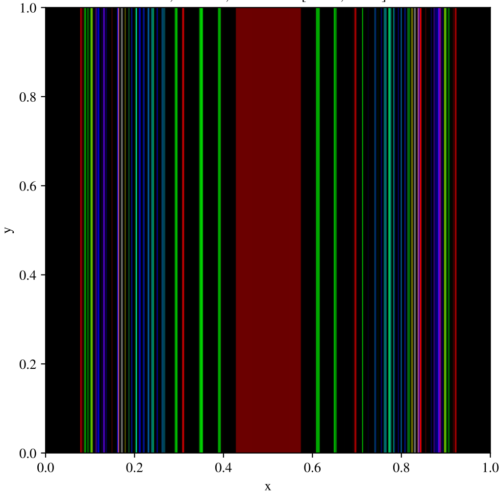
Toro test 2, x-split, Uniform (400x400) \rho , t = 0.15 , fixed scale [0.015, 1.000]
