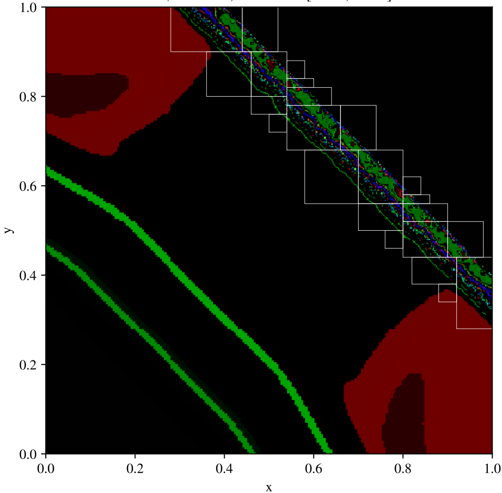
Toro test 3, diagonal split, AMR (base 200x200, max_level=1) \rho , t = 0.012 , fixed scale [0.446, 6.206]
