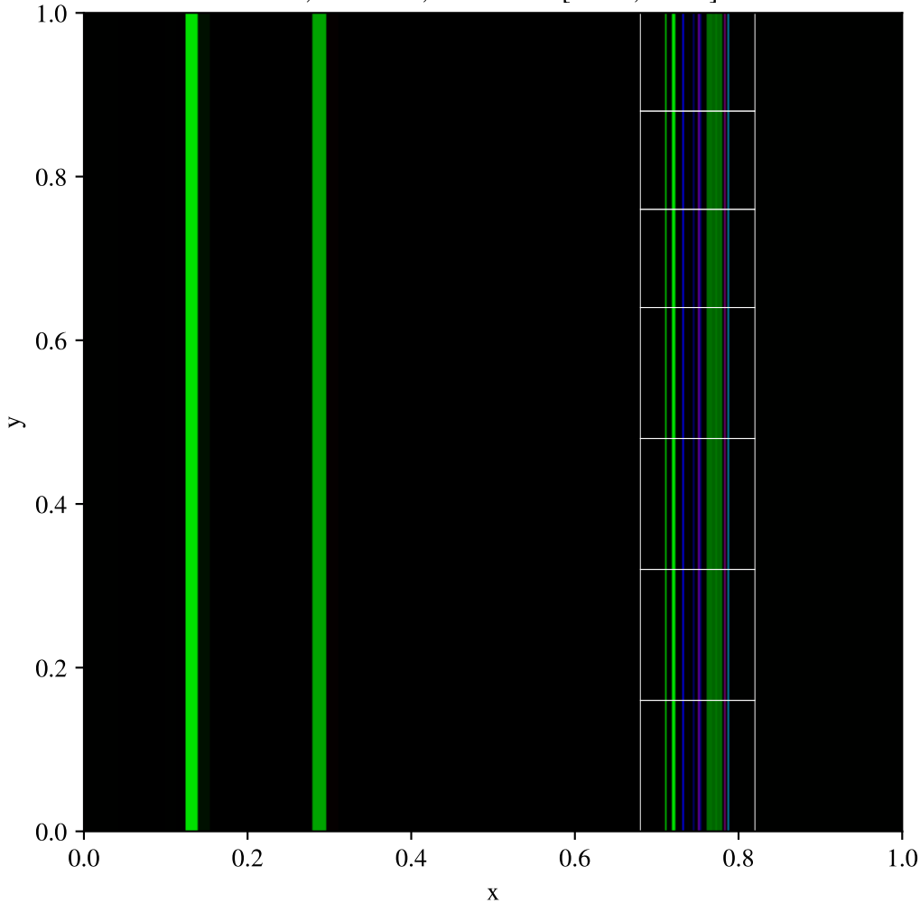
Toro test 3, x-split, AMR (base 200x200, max_level=1) \rho , t = 0.012 , fixed scale [0.446, 6.206]
