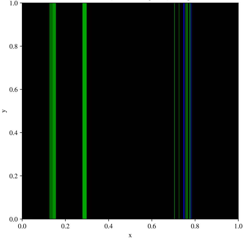
Toro test 3, x-split, Uniform (400x400) \rho , t = 0.012 , fixed scale [0.446, 6.206]
