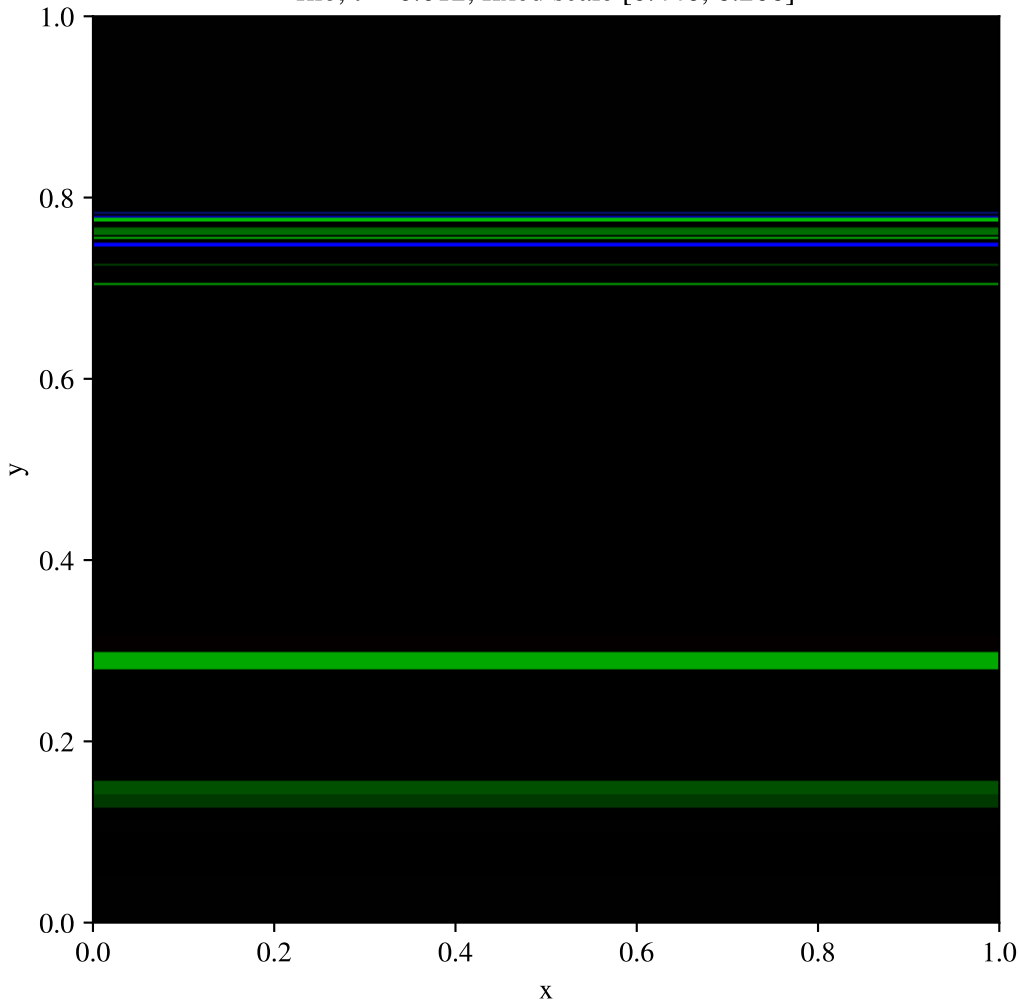
Toro test 3, y-split, Uniform (400x400) \rho , t = 0.012 , fixed scale [0.446, 6.206]
