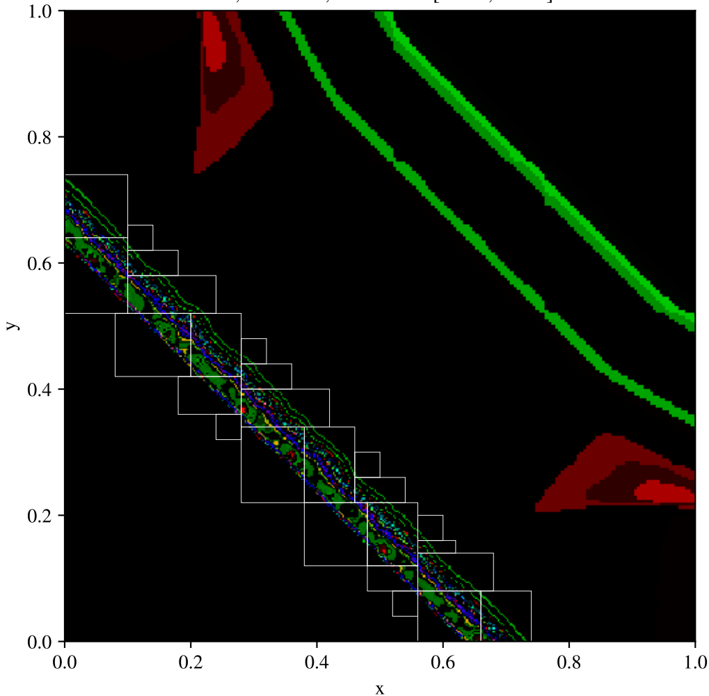
Toro test 4, diagonal split, AMR (base 200x200, max_level=1) \rho , t = 0.035 , fixed scale [0.455, 6.283]
