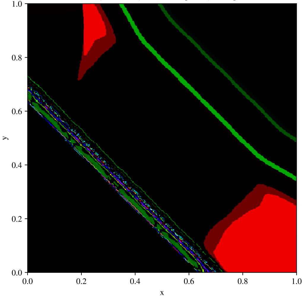
Toro test 4, diagonal split, Uniform (400x400) \rho, t = 0.035 , fixed scale [0.455, 6.283]
