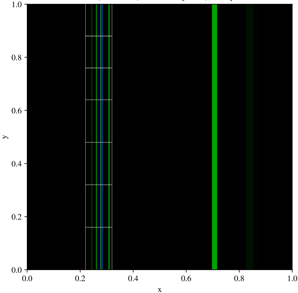
Toro test 4, x-split, AMR (base 200x200, max_level=1) \rho , t = 0.035 , fixed scale [0.455, 6.283]
