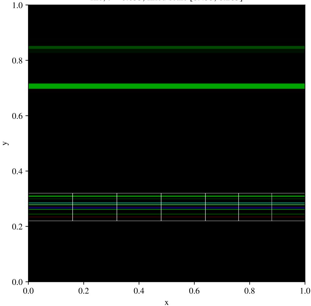
Toro test 4, y-split, AMR (base 200x200, max_level=1) \rho , t = 0.035 , fixed scale [0.455, 6.283]
