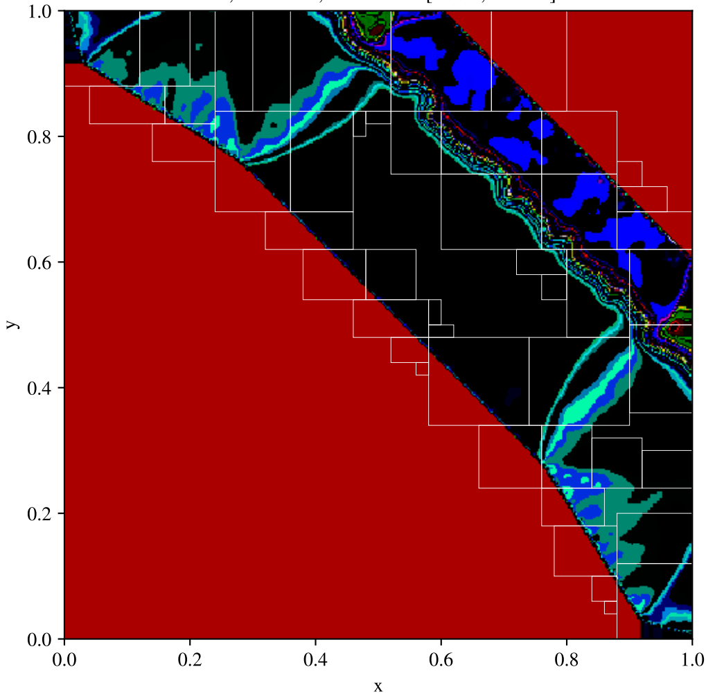
Toro test 5, diagonal split, AMR (base 200x200, max_level=1) \rho , t = 0.035 , fixed scale [5.992, 36.670]
