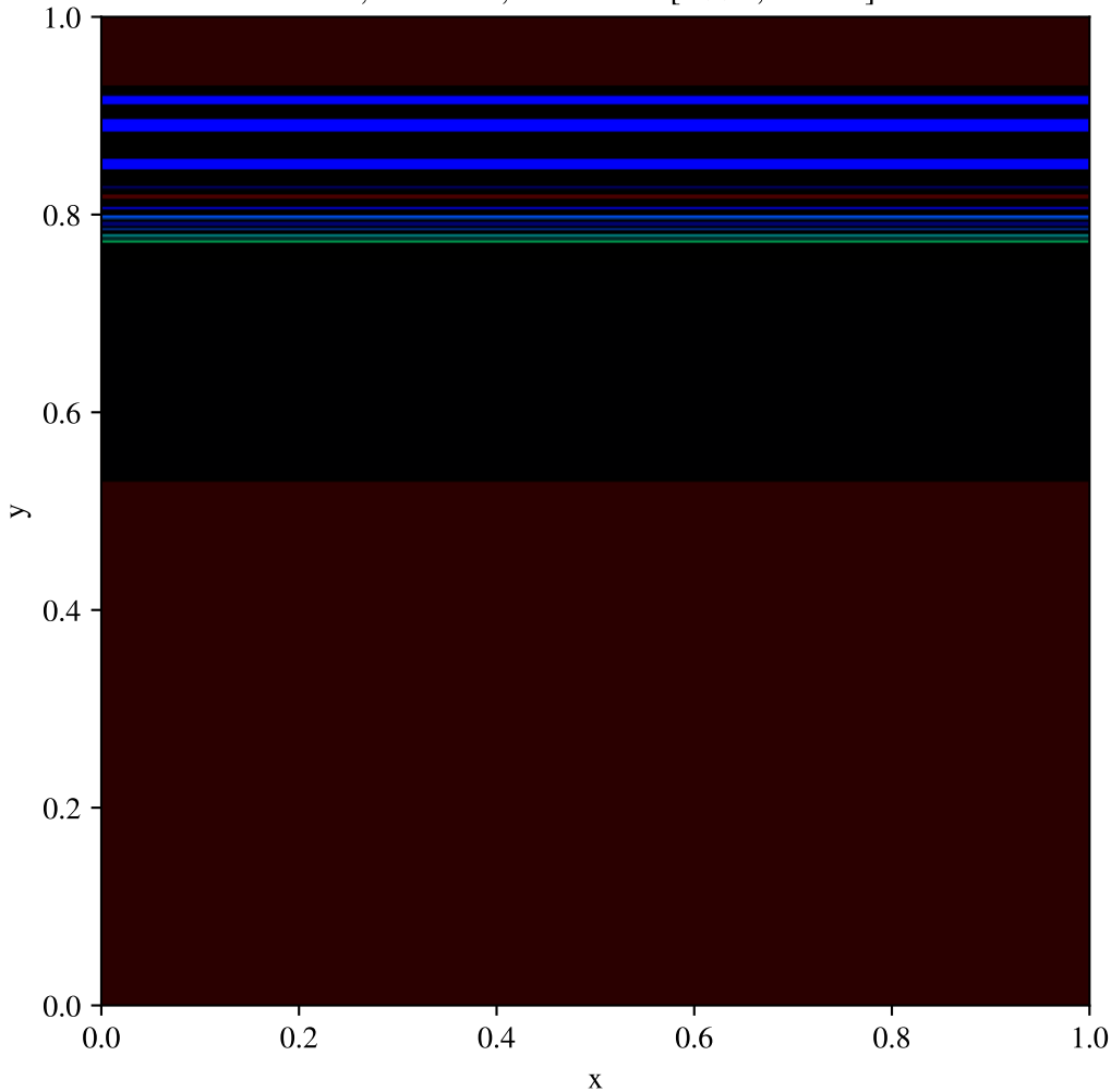
Toro test 5, y-split, Uniform (400x400) \rho , t = 0.035 , fixed scale [5.992, 36.670]
