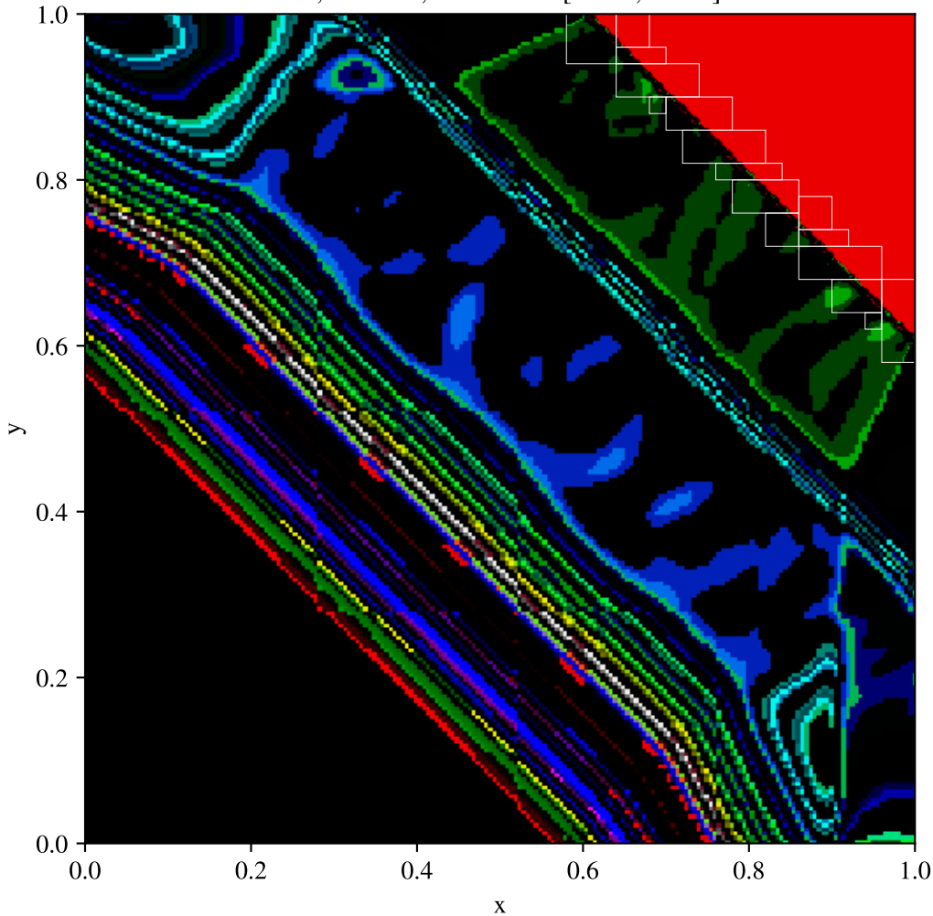
Toro test 1, diagonal split, AMR (base 200x200, max_level=1) \rho , t = 0.25 , fixed scale [0.125, 1.000]
