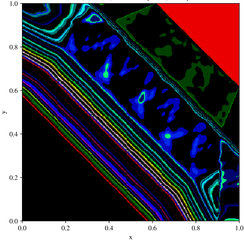
Toro test 1, diagonal split, Uniform (400x400) \rho , t = 0.25 , fixed scale [0.125, 1.000]
