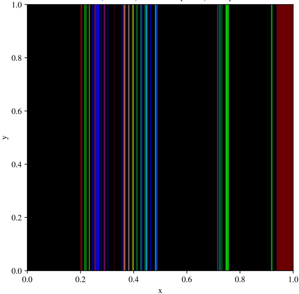
Toro test 1, x-split, Uniform (400x400) \rho , t = 0.25 , fixed scale [0.125, 1.000]
