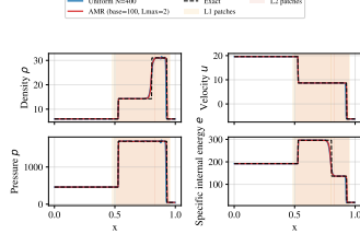
Toro Test 5: AMR vs Uniform at Matched Effective N=400 ( t = 0.035 )
