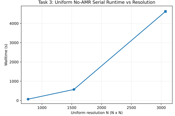
Figure 9: Uniform serial wall-clock runtime for the Task 3 quadrant problem at t_{\text{end}} = 0.3 as the grid is doubled from 768^2 to 3072^2 , showing the near-cubic cost growth discussed in the text.
