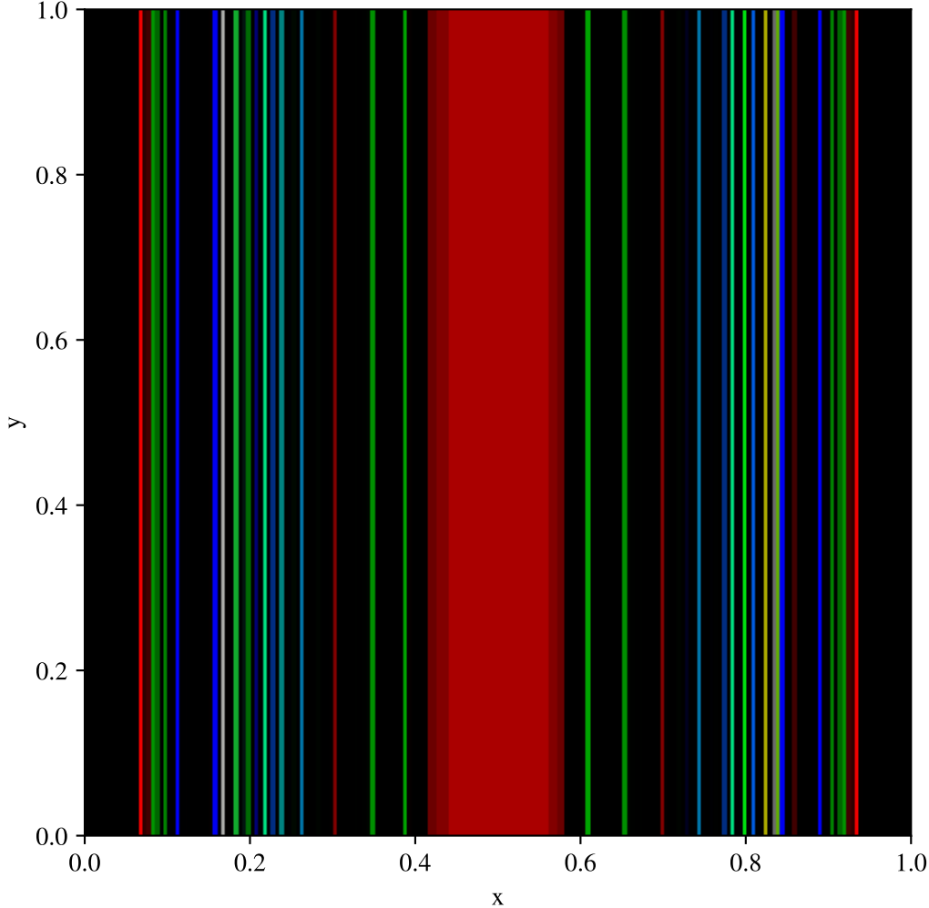
Toro test 2, x-split, AMR (base 200x200, max_level=1) \rho , t = 0.15 , fixed scale [0.015, 1.000]
