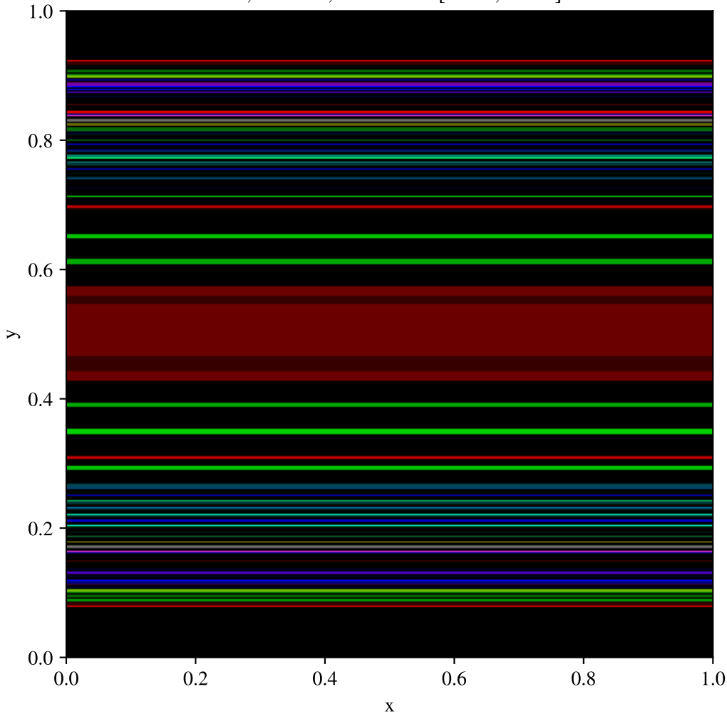
Toro test 2, y-split, Uniform (400x400) \rho , t = 0.15 , fixed scale [0.015, 1.000]
