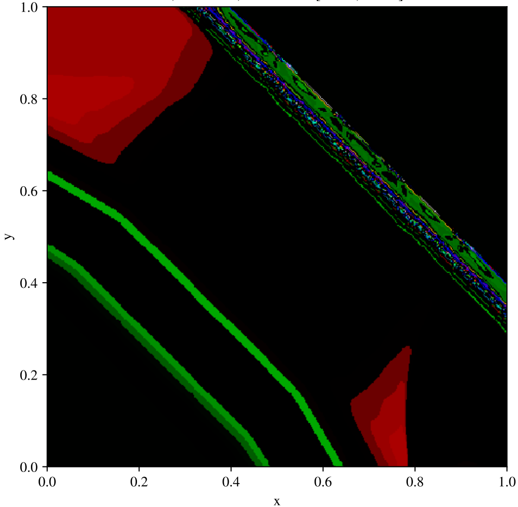
Toro test 3, diagonal split, Uniform (400x400) \rho , t = 0.012 , fixed scale [0.446, 6.206]
