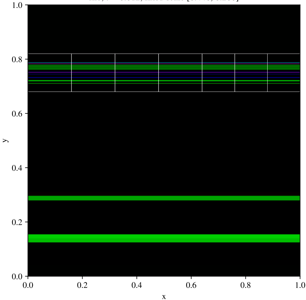
Toro test 3, y-split, AMR (base 200x200, max_level=1) \rho , t = 0.012 , fixed scale [0.446, 6.206]
