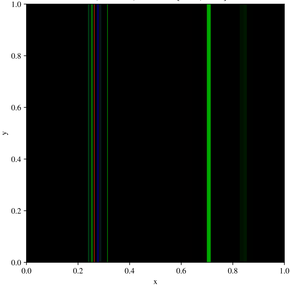
Toro test 4, x-split, Uniform (400x400) \rho , t = 0.035 , fixed scale [0.455, 6.283]
