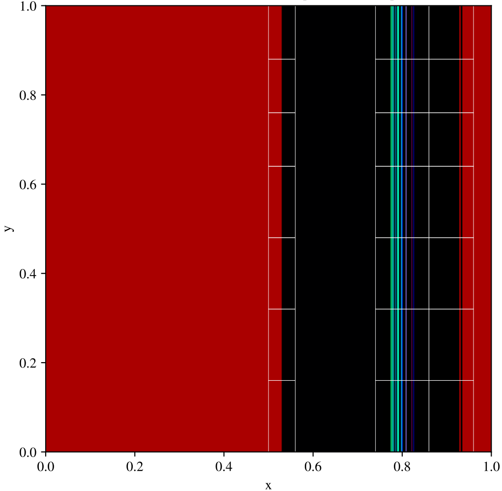
Toro test 5, x-split, AMR (base 200x200, max_level=1) \rho , t = 0.035 , fixed scale [5.992, 36.670]
