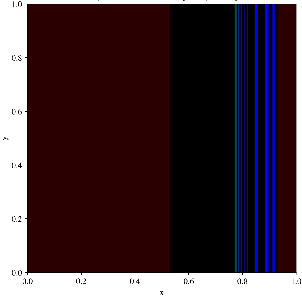
Toro test 5, x-split, Uniform (400x400) \rho , t = 0.035 , fixed scale [5.992, 36.670]
