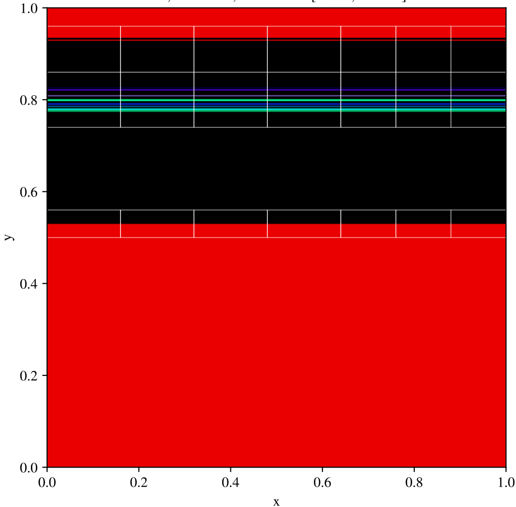
Toro test 5, y-split, AMR (base 200x200, max_level=1) \rho , t = 0.035 , fixed scale [5.992, 36.670]
