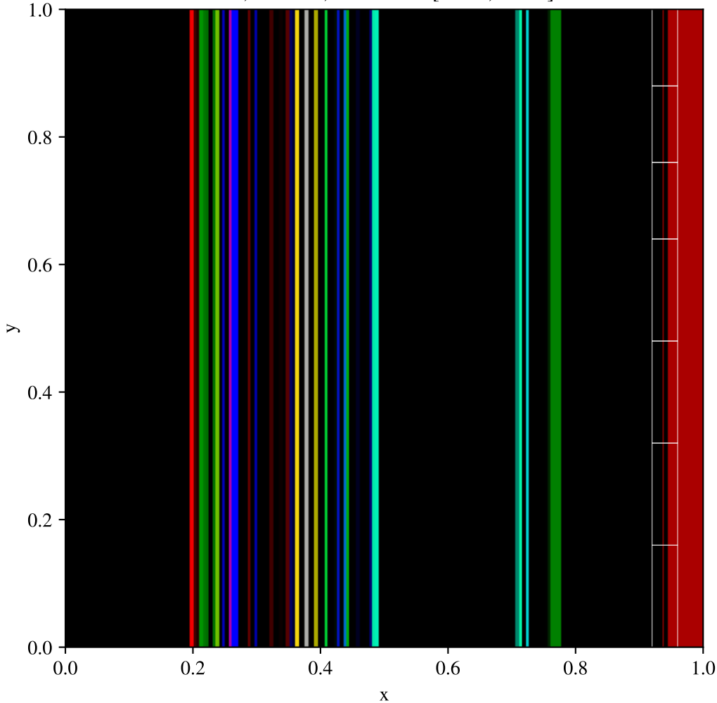
Toro test 1, x-split, AMR (base 200x200, max_level=1) \rho , t = 0.25 , fixed scale [0.125, 1.000]
