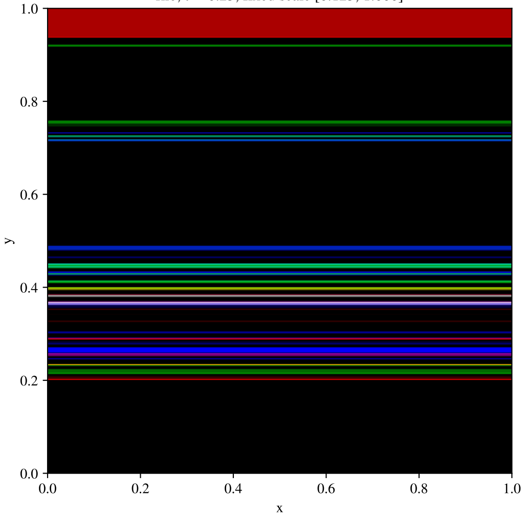
Toro test 1, y-split, Uniform (400x400) \rho , t = 0.25 , fixed scale [0.125, 1.000]
