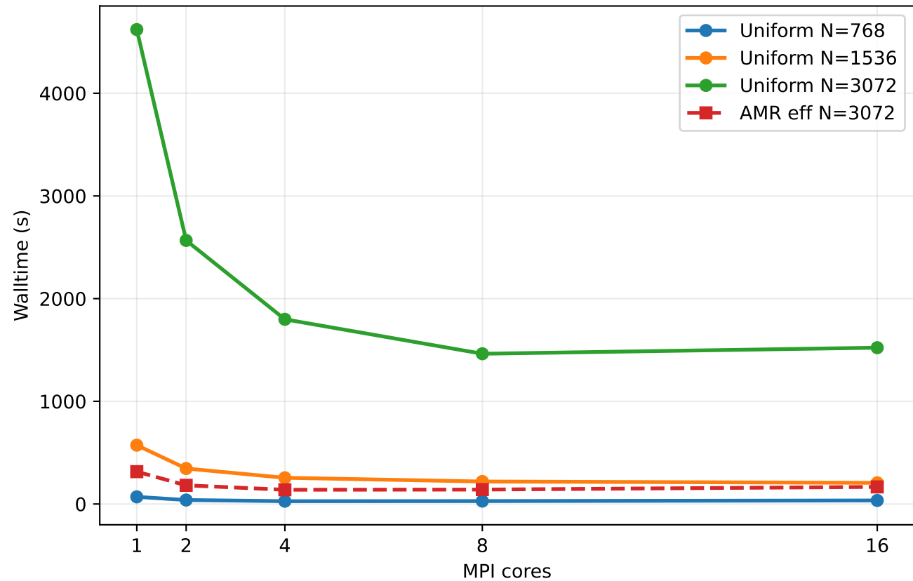
Task 3: Runtime vs Cores
