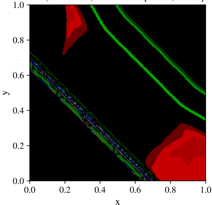
Toro test 4, diagonal split, Uniform (400x400) \rho , t = 0.035 , fixed scale [0.455, 6.283]
