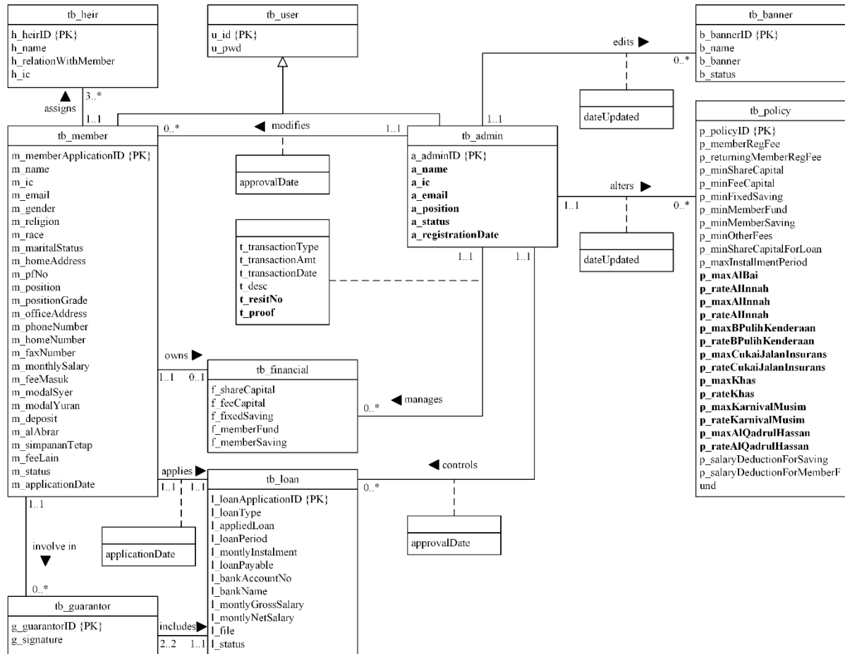
Figure 7 Conceptual ERD for the Proposed Module
