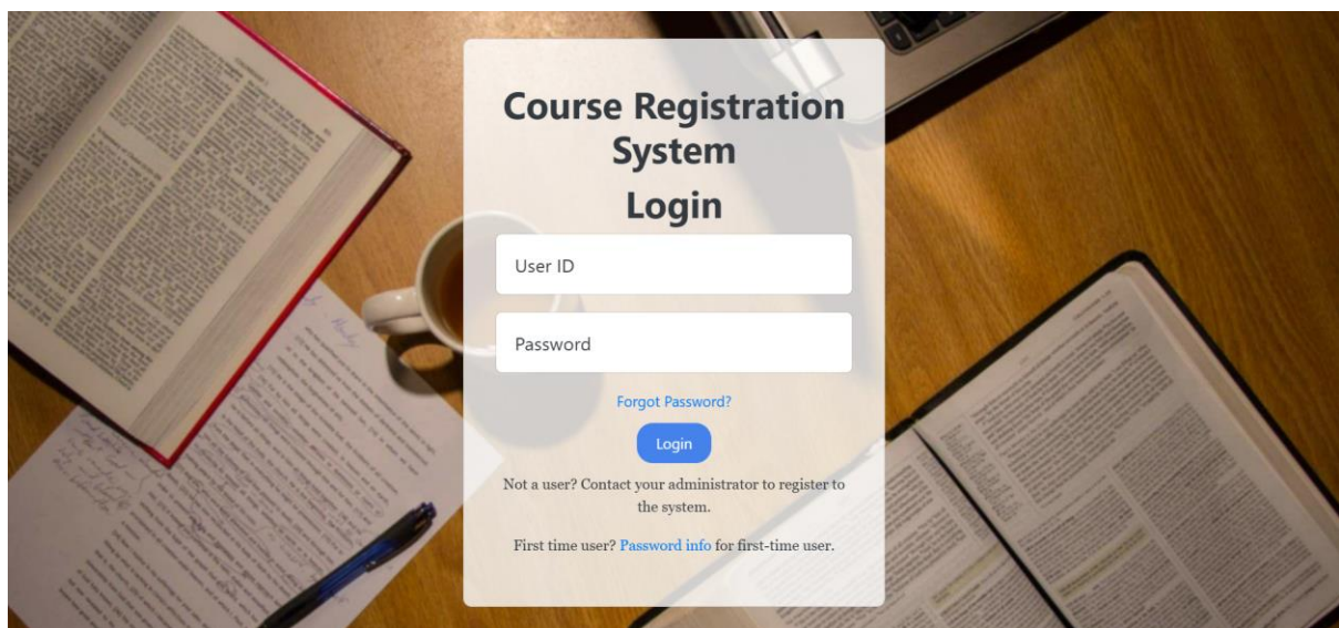
Figure 4 Login Page
