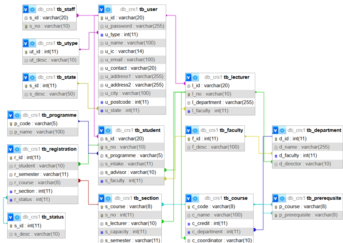
Figure 3 Database Structure and Relationship
