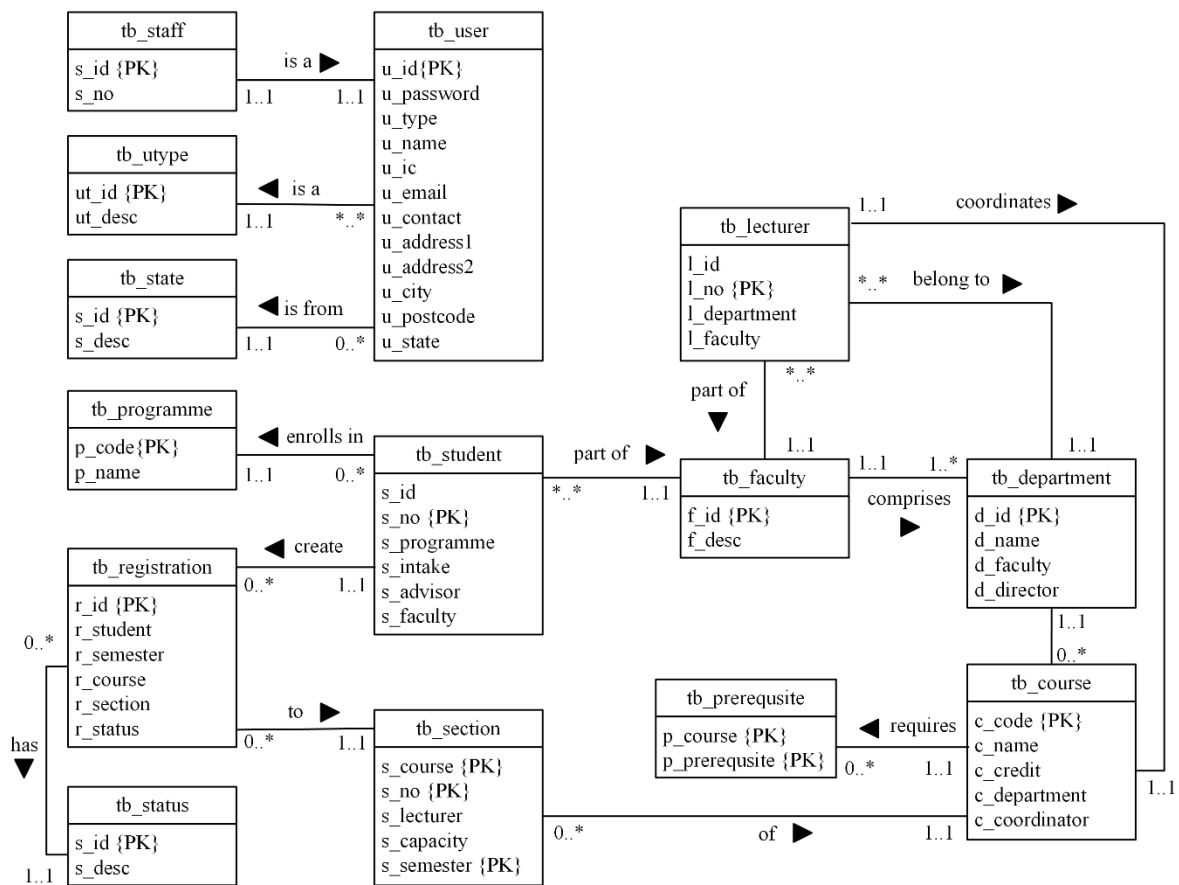
Figure 2 Entity Relationship Diagram for Course Registration System
