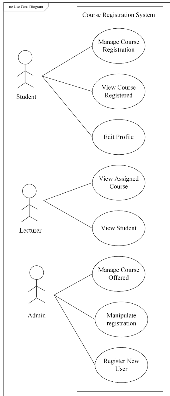
Figure 1 Use Case Diagram for Course Registration System
