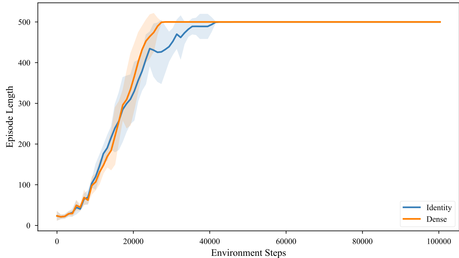
PPO Episode Lengths during Training on CartPole-v1
