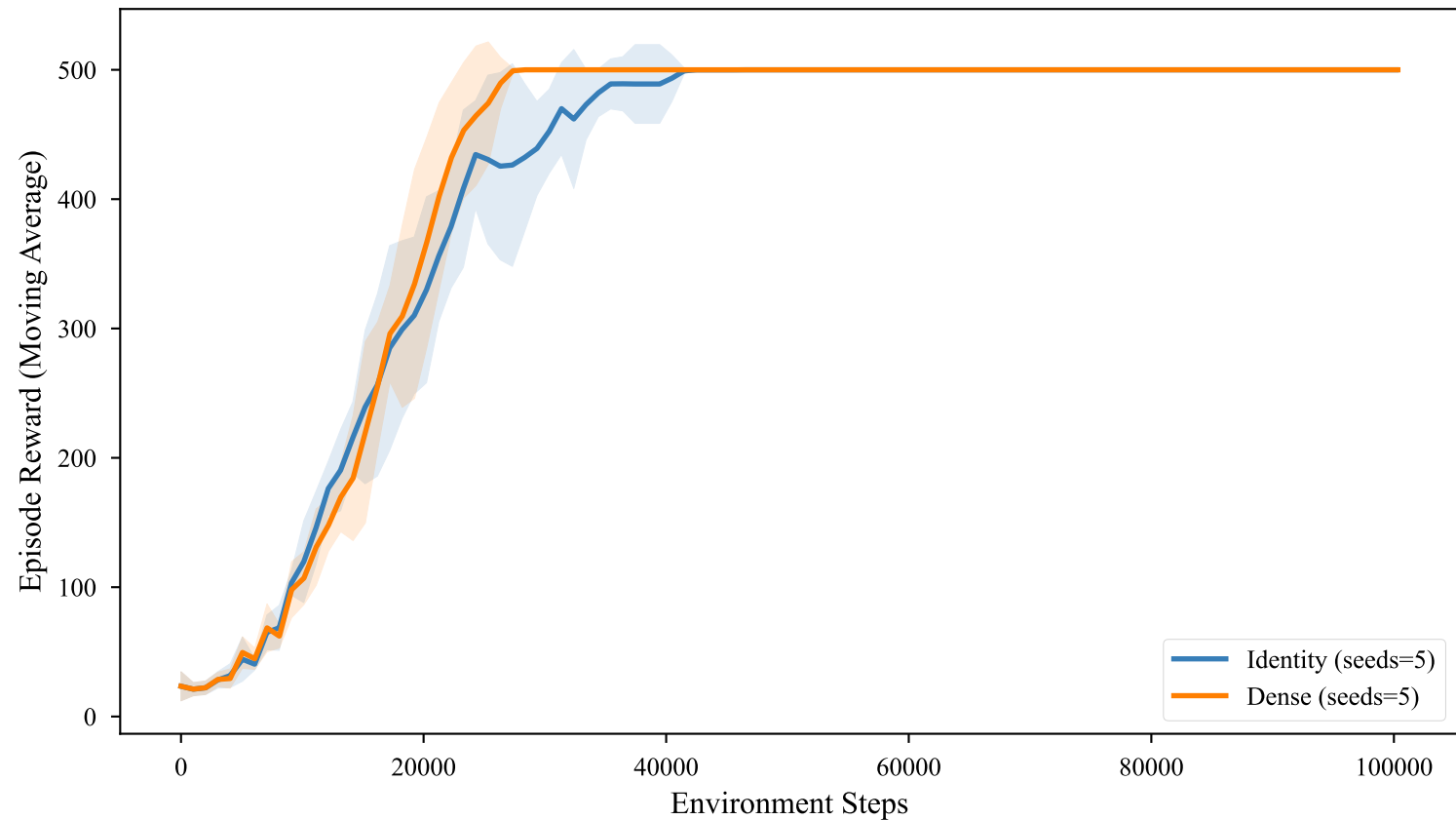
PPO Training Performance on CartPole-v1 (True Unshaped Objective)
