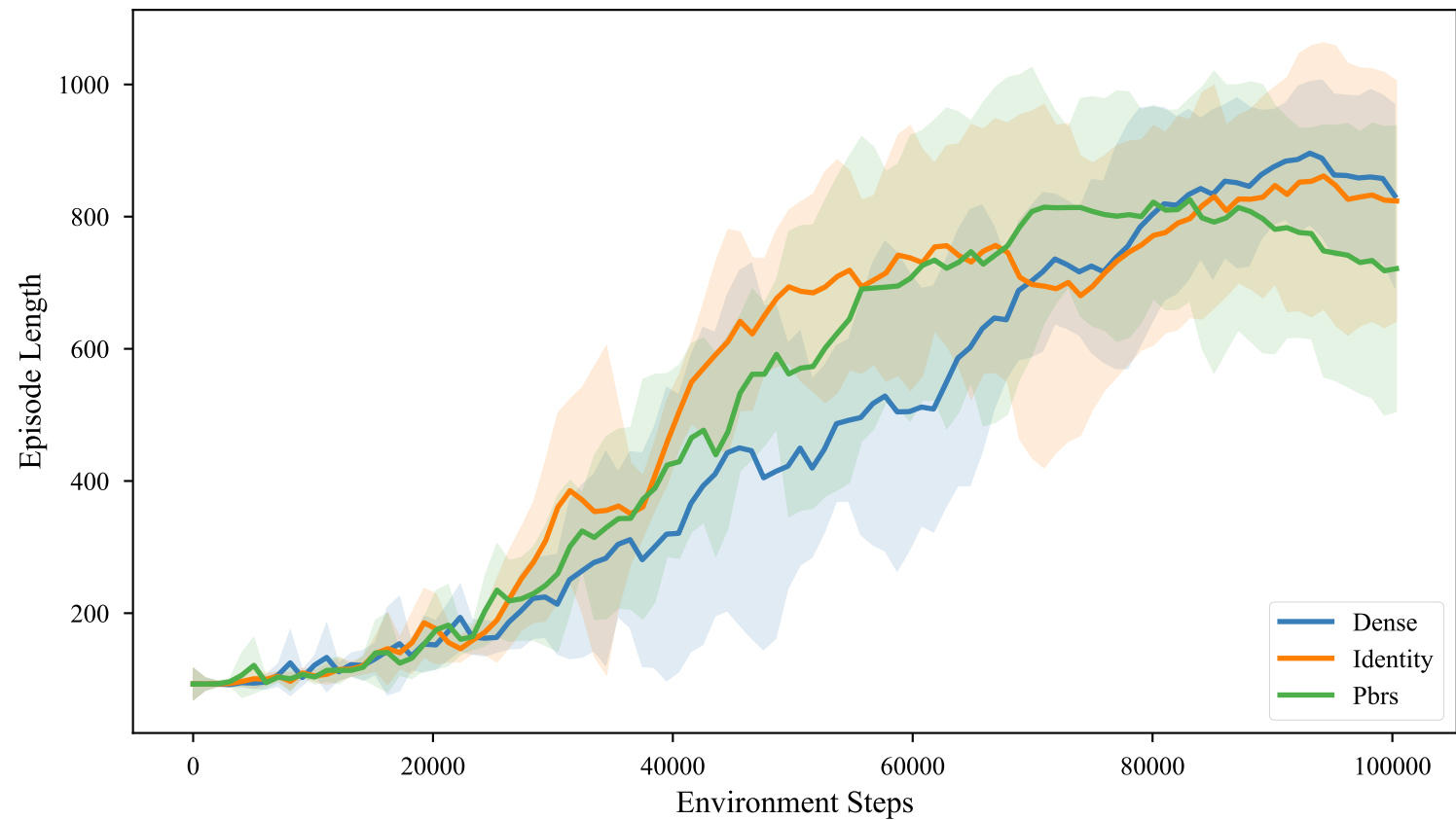
PPO Episode Lengths during Training on LunarLander-v3
