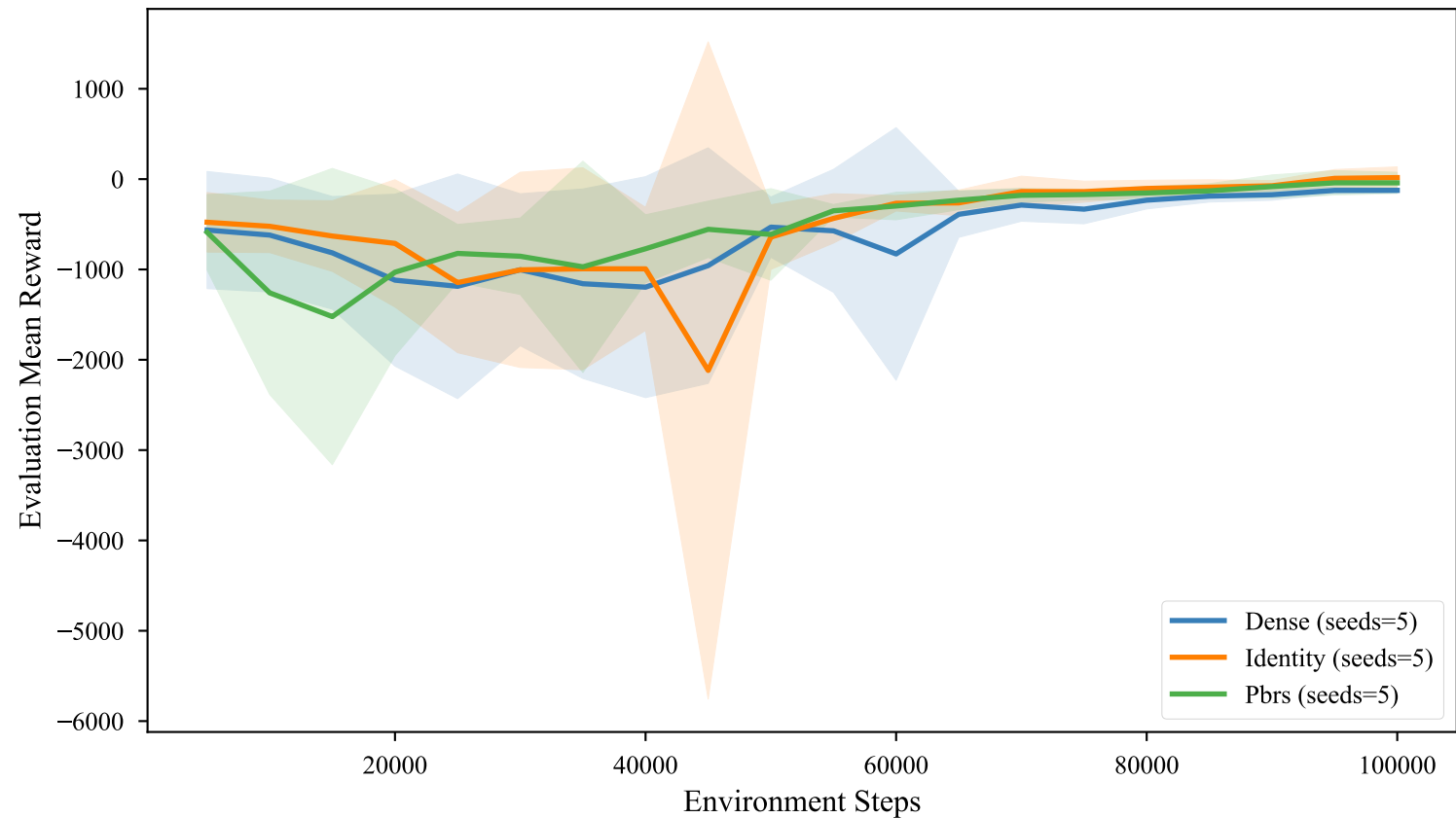
PPO Evaluation Performance on LunarLander-v3 (Deterministic, Unshaped)
