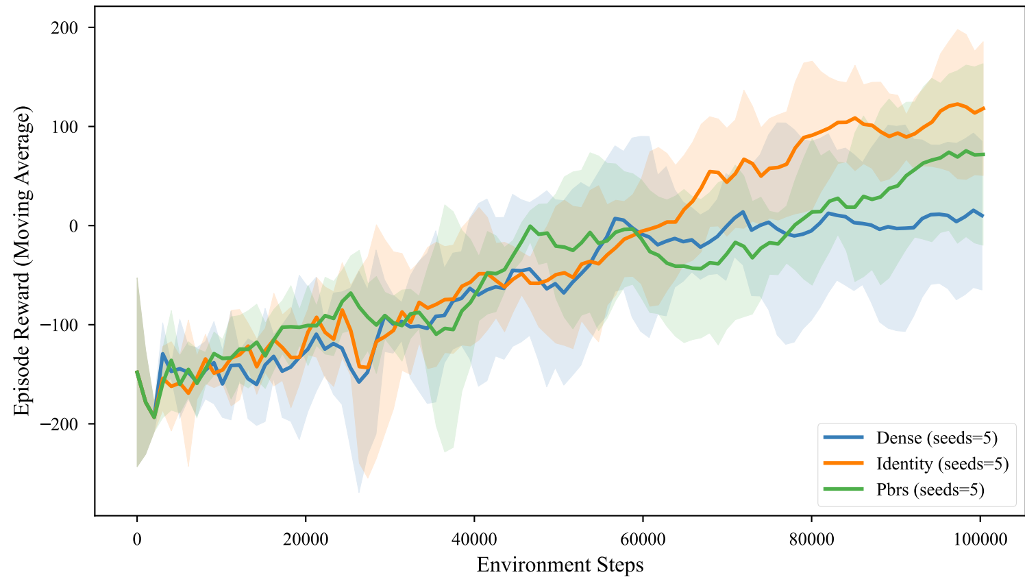
PPO Training Performance on LunarLander-v3 (True Unshaped Objective)
