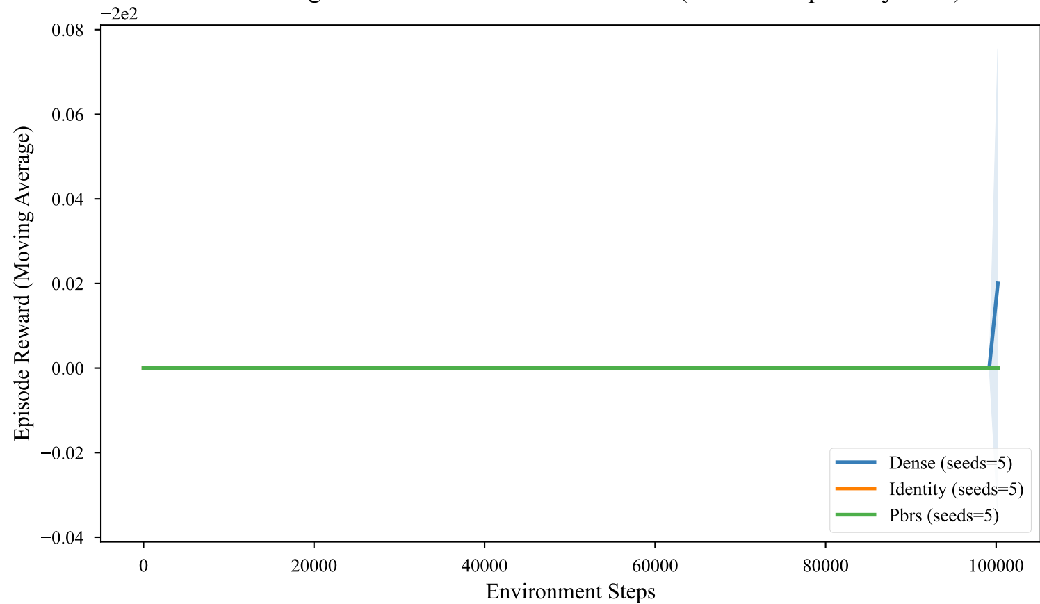
PPO Training Performance on MountainCar-v0 (True Unshaped Objective)
