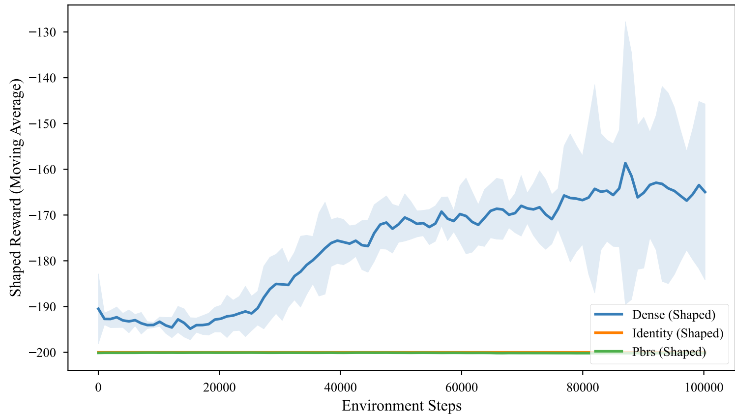
PPO Training Performance on MountainCar-v0 (Proxy Shaped Objective)
