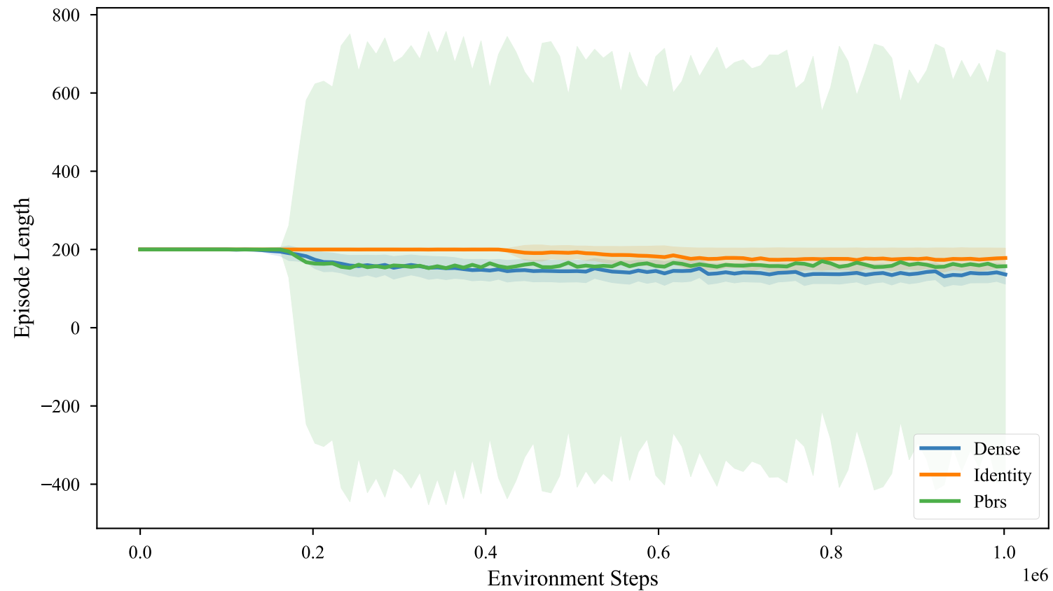
PPO Episode Lengths during Training on MountainCar-v0
