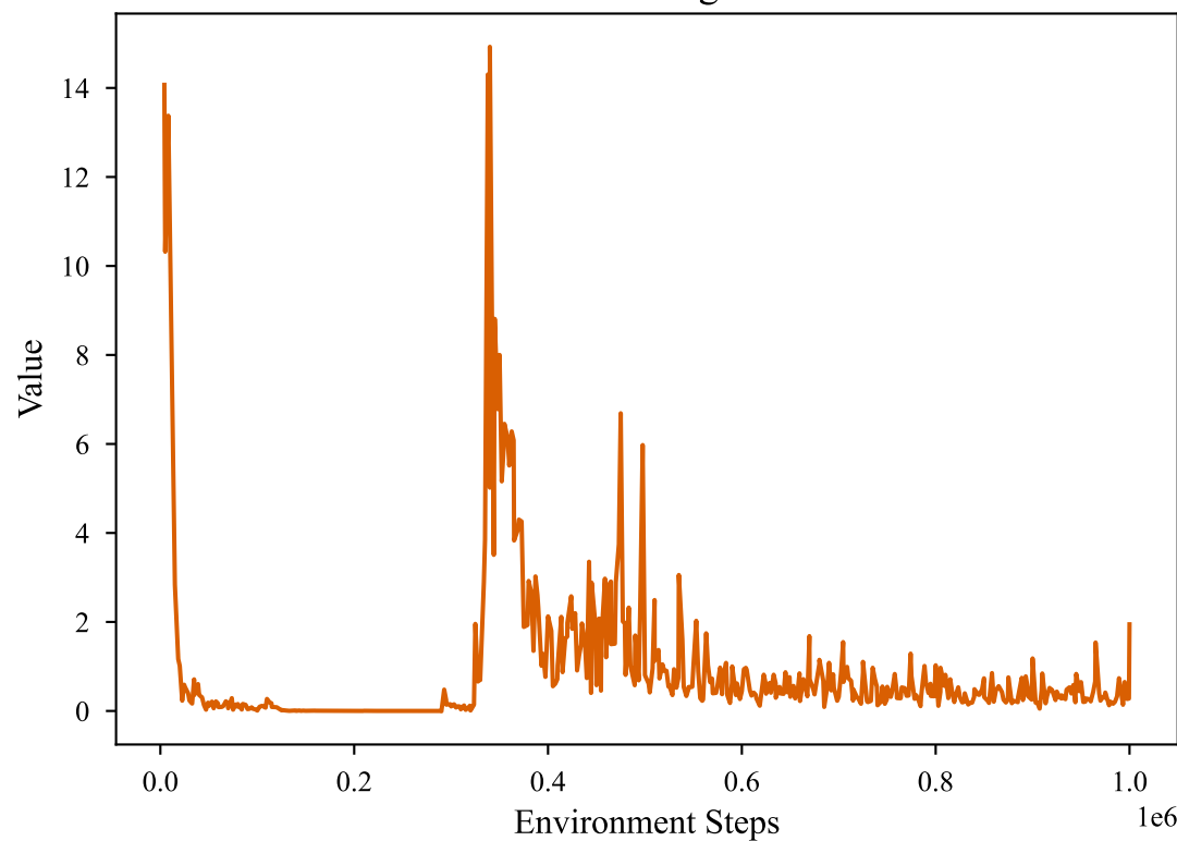
Policy Gradient Loss
