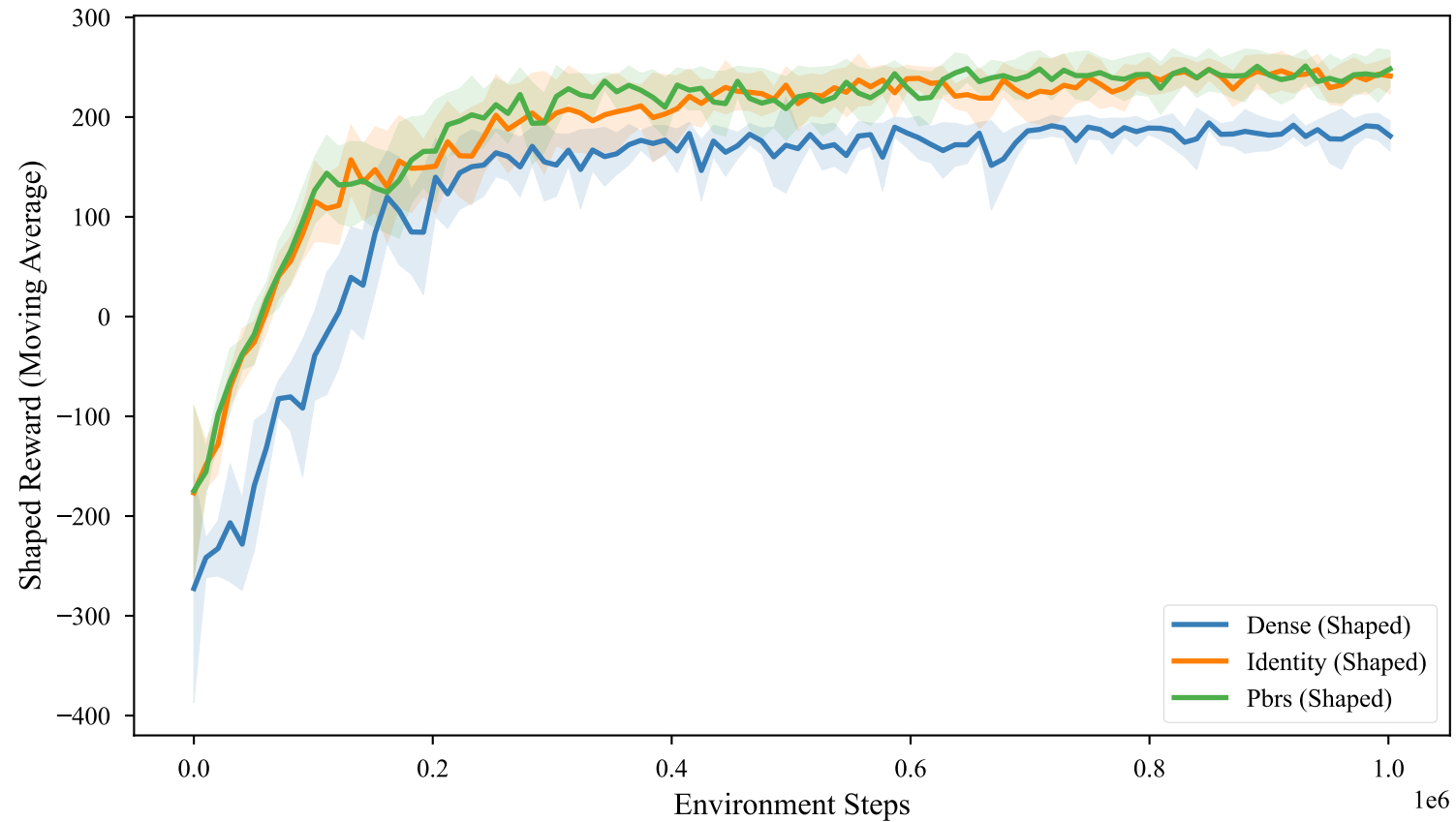
PPO Training Performance on LunarLander-v3 (Proxy Shaped Objective)
